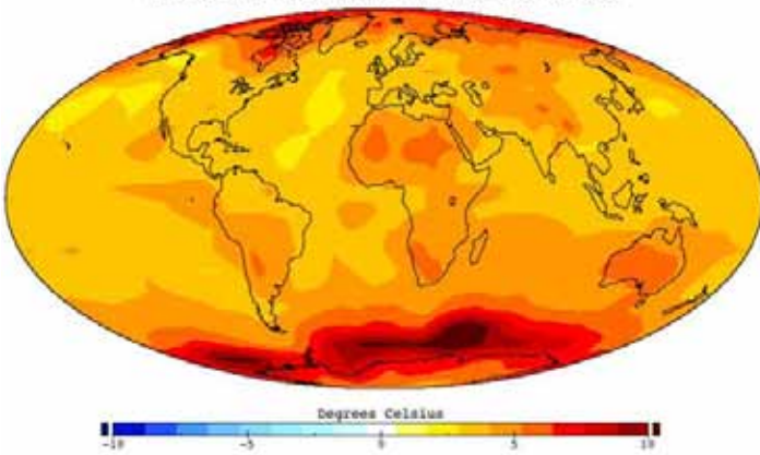
Surface Air Temperature Increase 1960 to 2060
