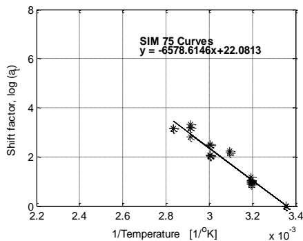
Figure 14. Arrhenius plot of SIM curves at 75% ABL
