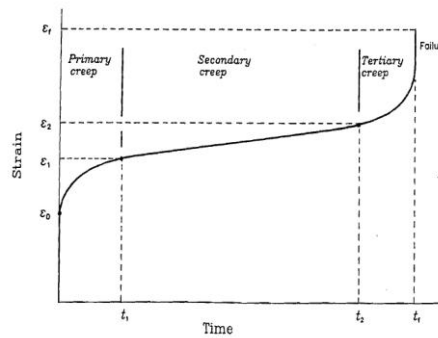
Figure 13. Schematic creep curve (Guimaraes, 1988)
